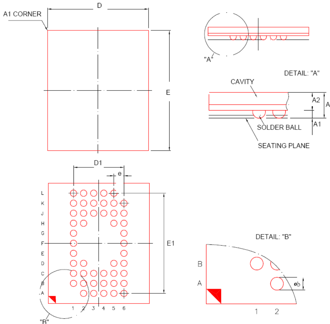
FIGURE 16. 48L WFBGA 5mm x 6mm package outline
