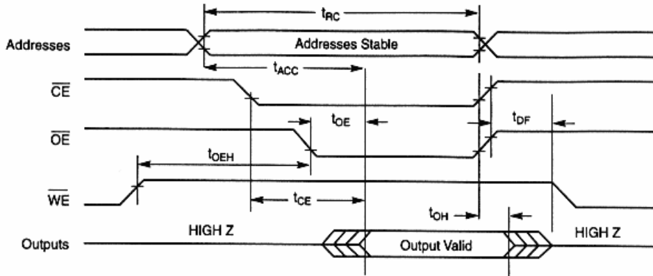
Figure 5. AC Waveforms for READ Operations
