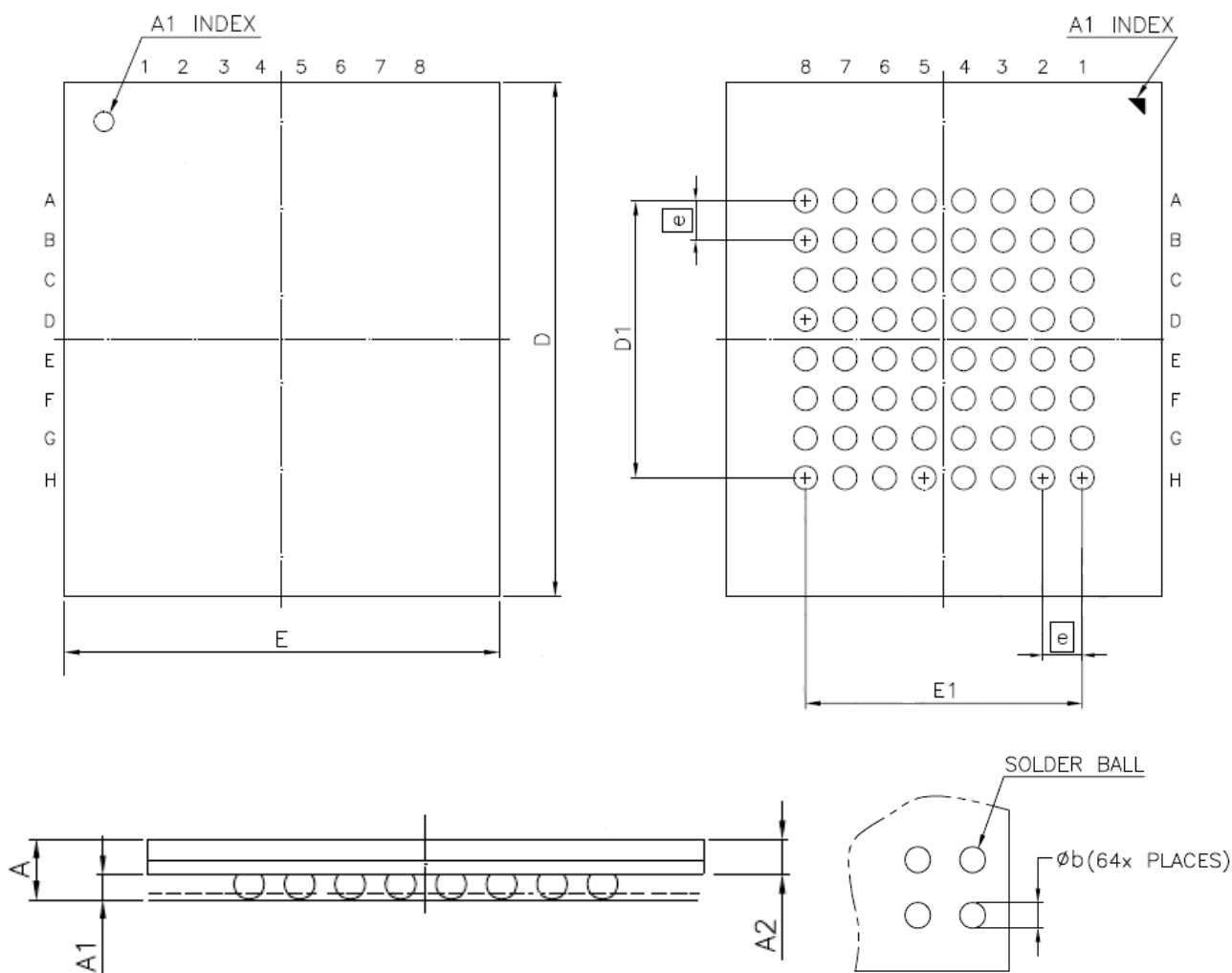
FIGURE 21. 64-ball Ball Grid Array (FBGA), 11 X13 mm, Pitch 1mm package outline
