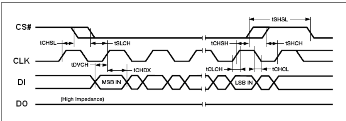
Figure 38. Input Timing
