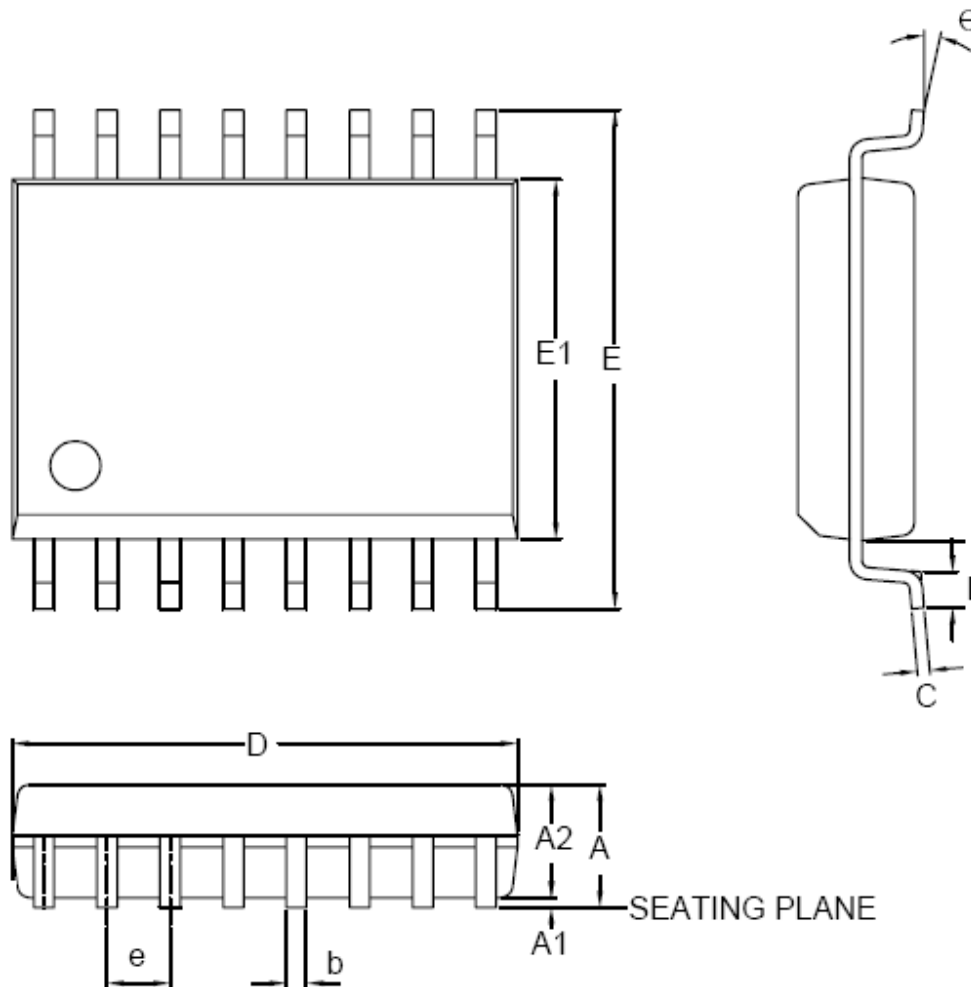
Figure 32. 16 LEAD SOP 300 mil
