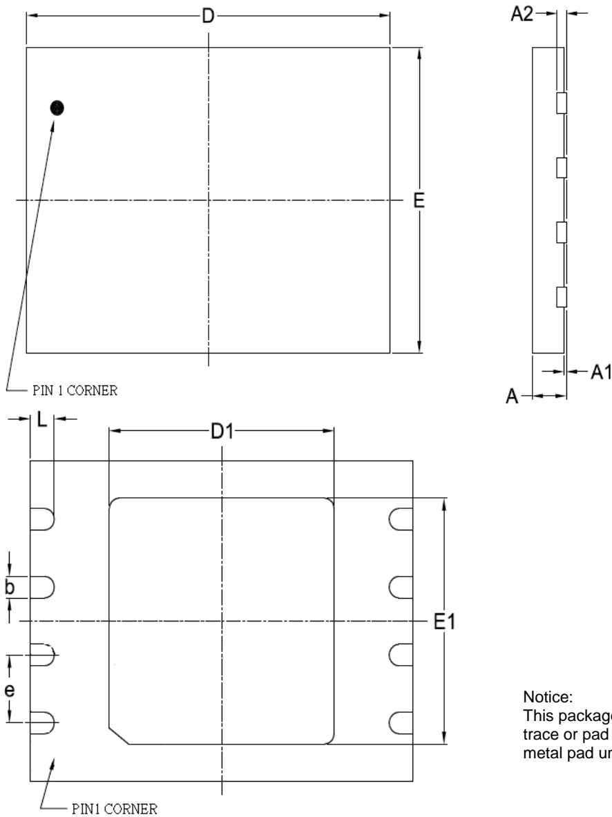
Figure 31. VDFN 8 ( 6x8 mm )
