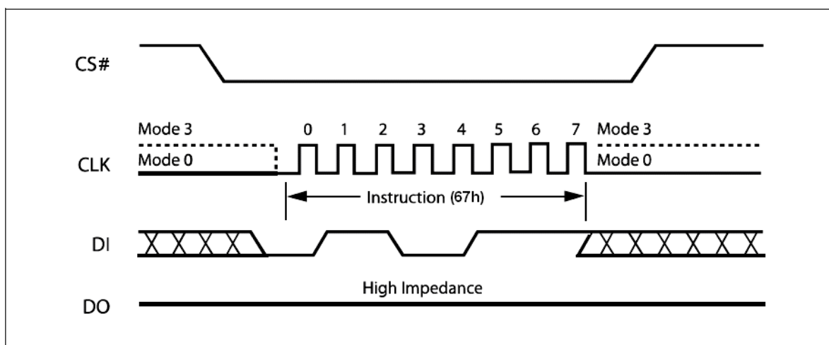
Figure 14. Enter High Bank Latch mode Instruction Sequence Diagram
