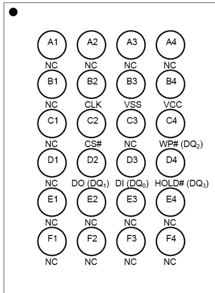
24 - Ball BGA
