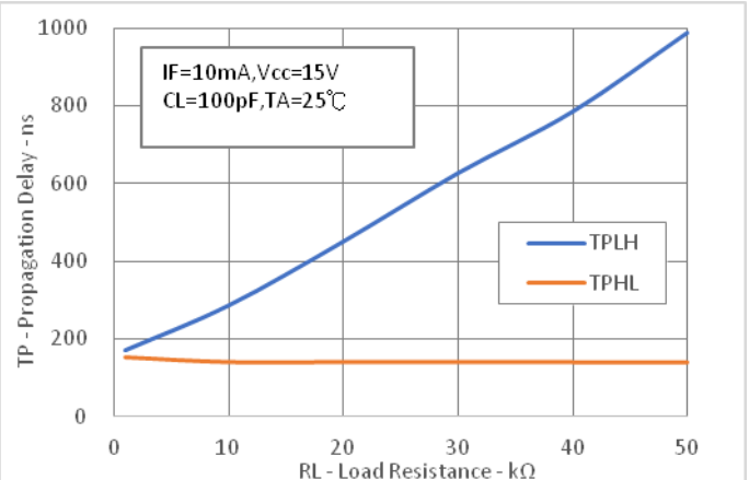
Fig.6 Propagation Delay vs. Load Resistance
