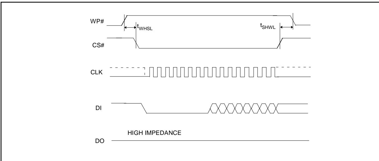
Figure 45. Write Protect setup and hold timing during WRSR when SRP = 1
