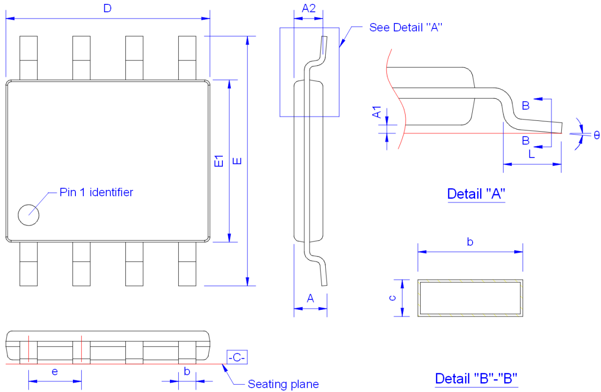
Figure 47. 8-pin VSOP (150mil)
