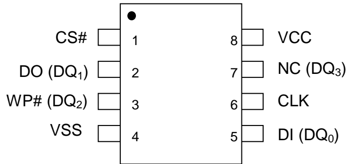
Figure.1 CONNECTION DIAGRAMS (TOP VIEW)
