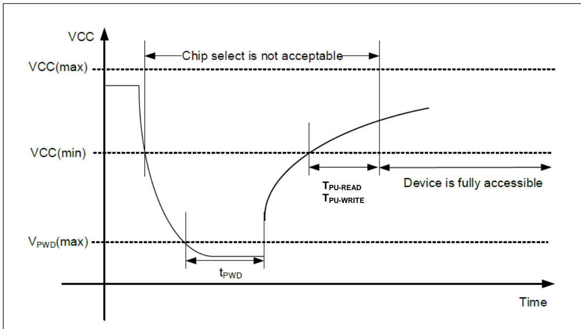
Figure 40. Power-down Timing
