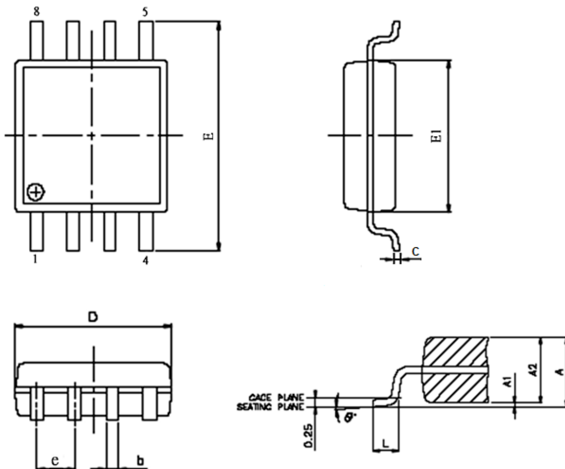
Figure 36. 8-pin SOP 200 mil (official name = 208 mil)
