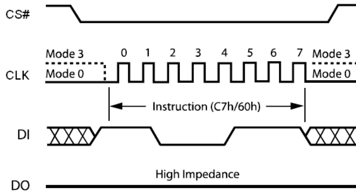
Figure 23. Chip Erase Instruction Sequence Diagram
