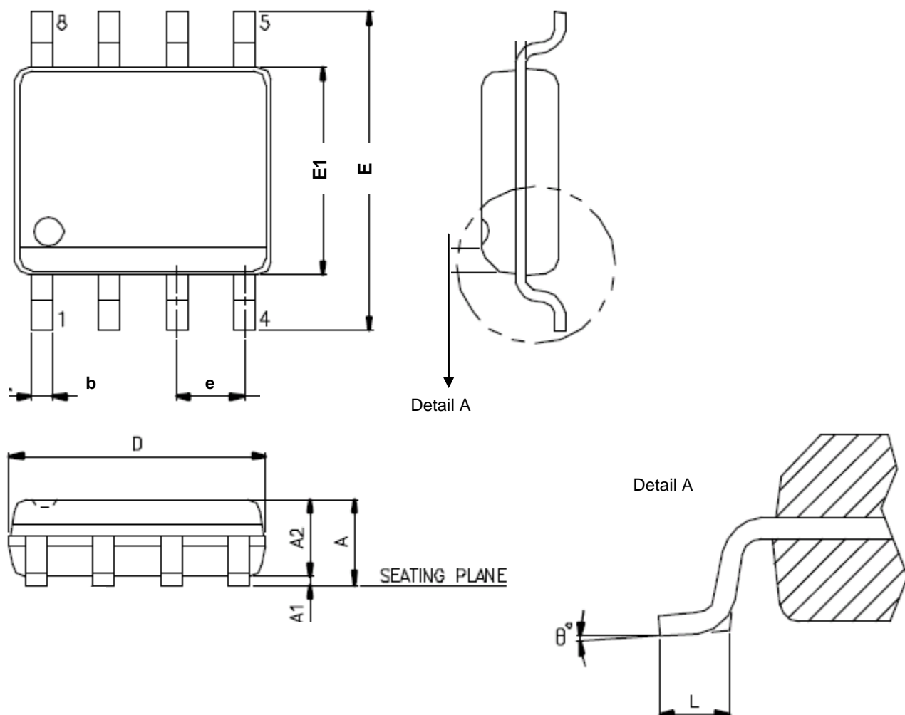
Figure 35. 8-pin SOP (150 mil)
