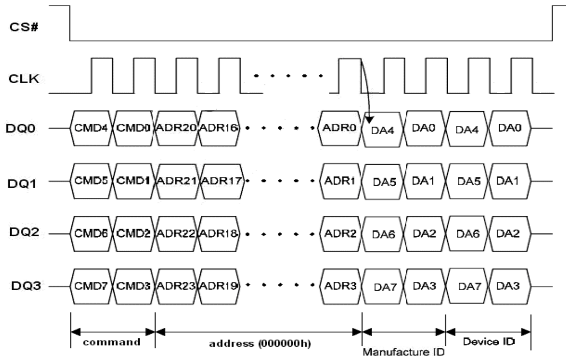
Figure 27. Read Manufacturer / Device ID Diagram
