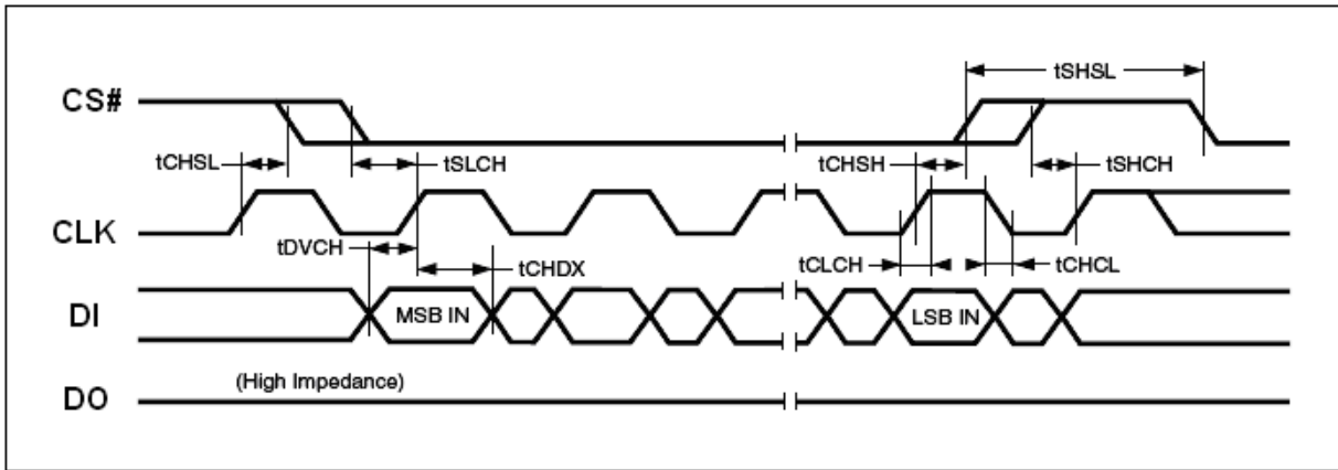
Input Timing
