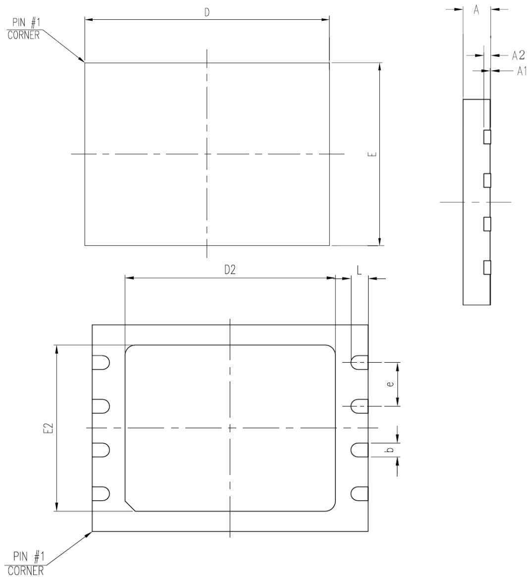
Figure 47. 8-contact VDFN / WSON (6x5mm)
