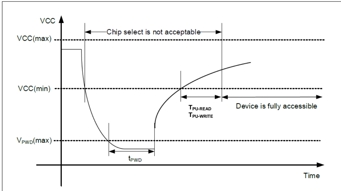
Figure 40. Power-down Timing
