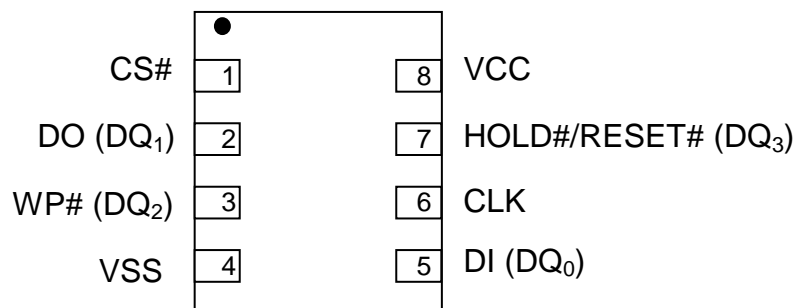
8 - LEAD VDFN / WSON / USON
