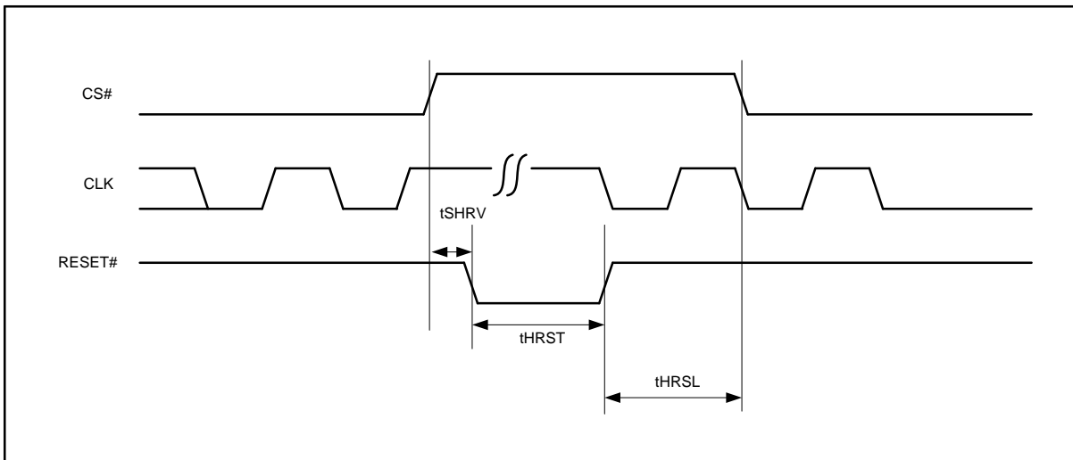
Figure 45. Reset Timing
