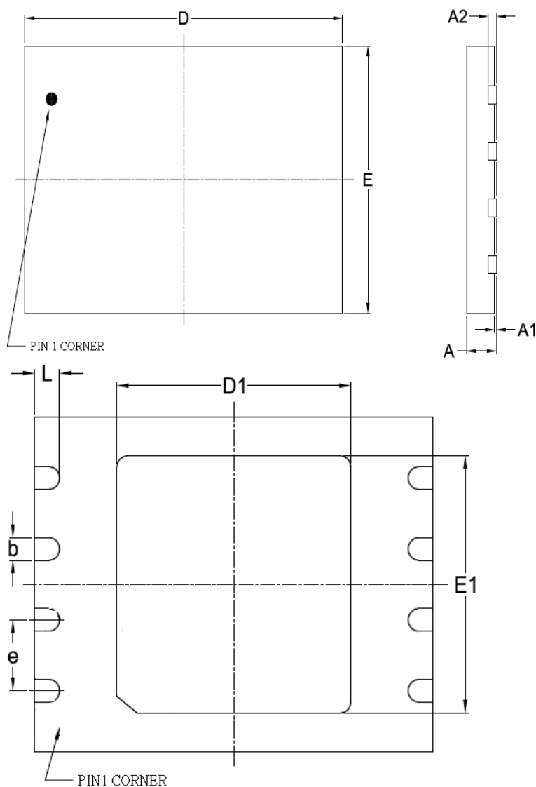
Figure 51. 8-contact VDFN / WSON (8x6mm)
