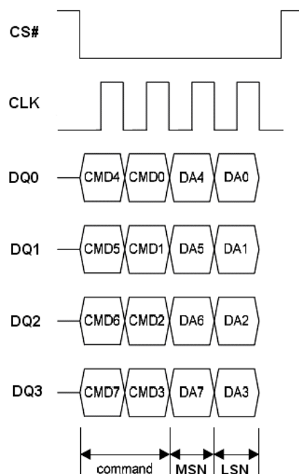
Figure 22. Write Status Register 3 Instruction Sequence Diagram
