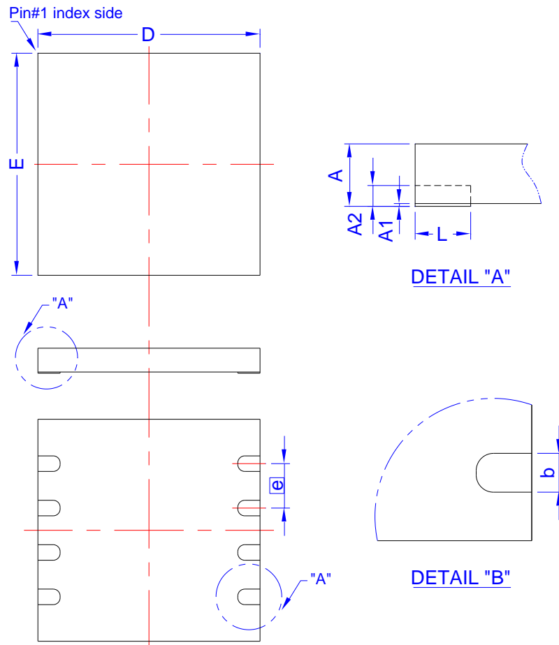
Figure 53. 8-contact USON (4x4x0.45 mm)
