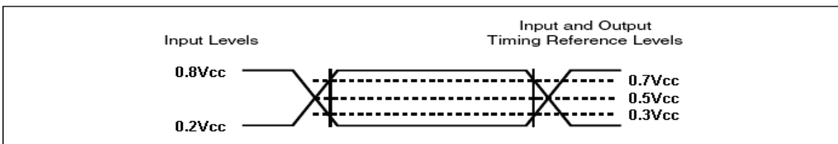
Figure 41. AC Measurement I/O Waveform
