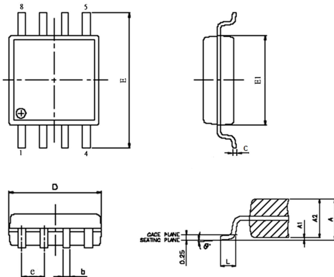
Figure 46. 8-pin SOP 200 mil (official name = 208 mil)
