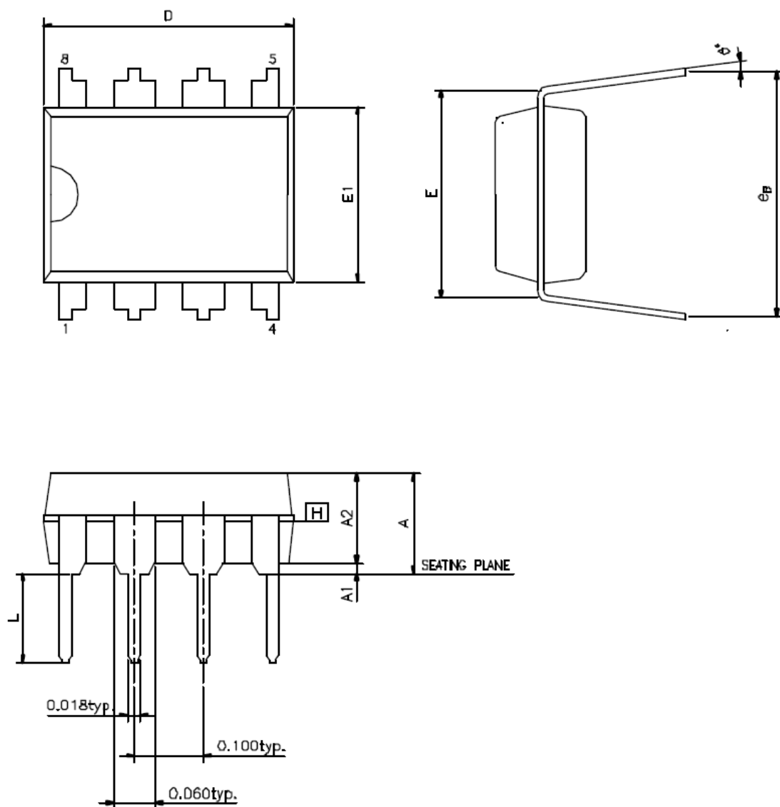
Figure 48. 8-pin PDIP
