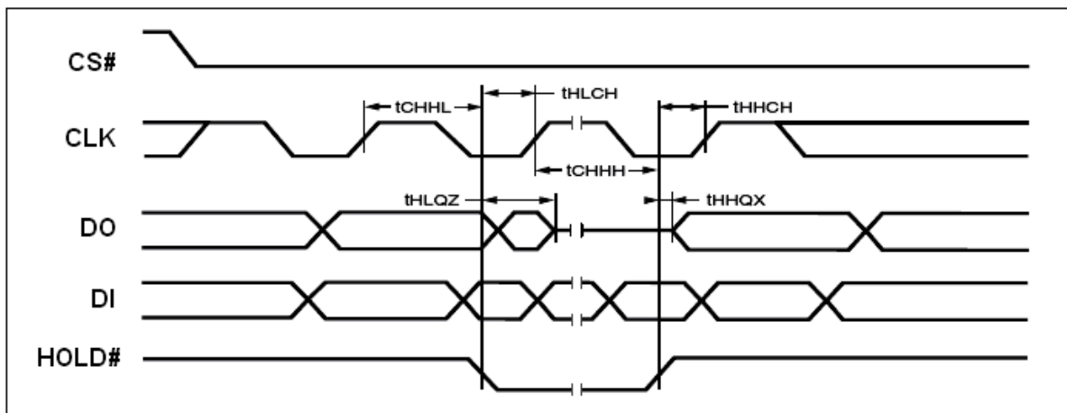
Figure 38. Hold Timing
