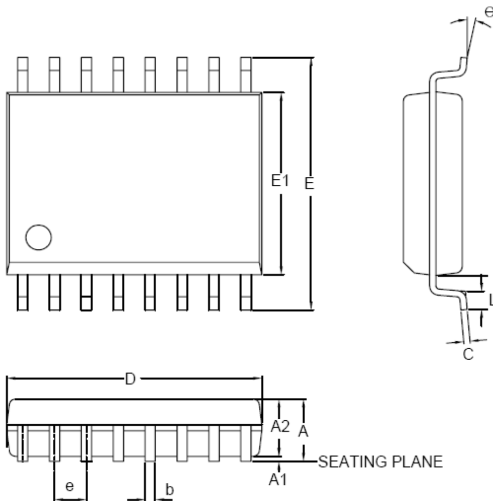
Figure 42. 16 LEAD SOP 300 mil
