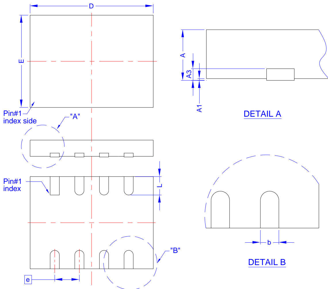
Figure 45. 8-contact USON (4x3x0.55 mm)
