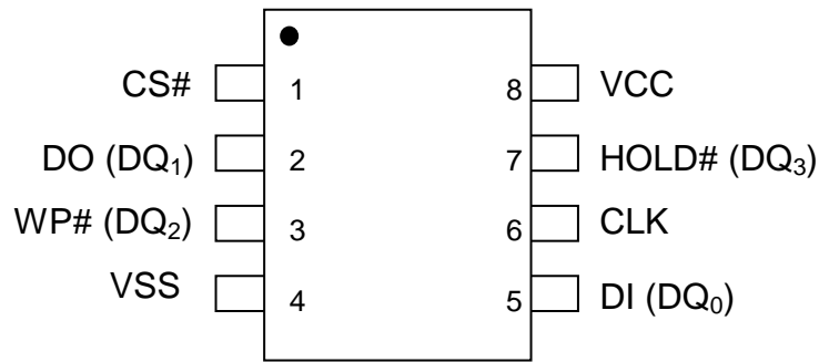
8 - LEAD SOP / PDIP
