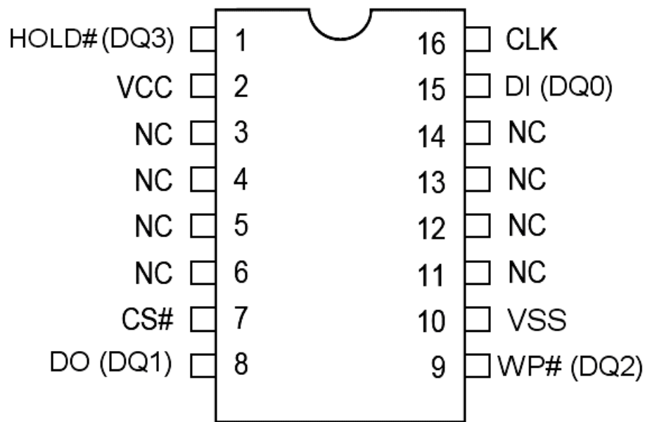
16 - LEAD SOP
