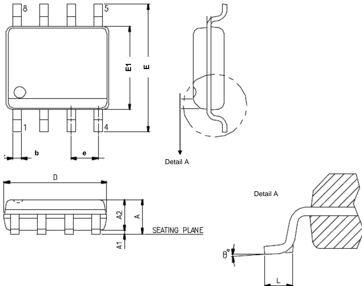
Figure 40. 8-pin SOP (150 mil)
