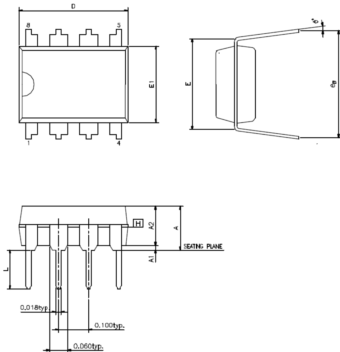
Figure 44. 8-pin PDIP
