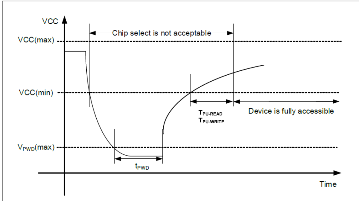
Figure 34. Power-down Timing
