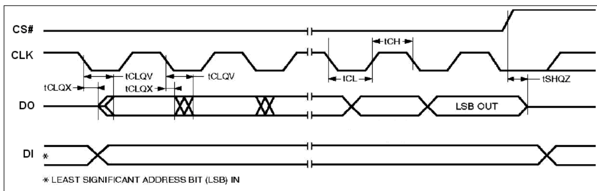
Figure 36. Serial Output Timing
