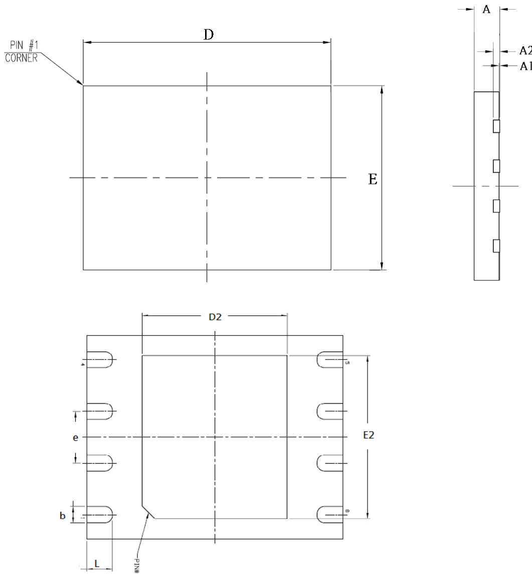
Figure 43. 8-contact VDFN / WSON (5x6 mm)
