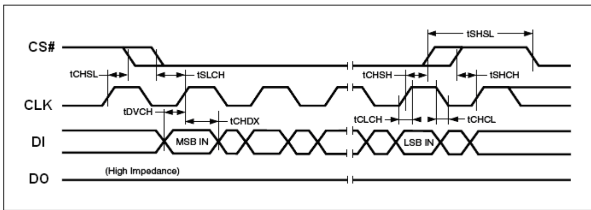
Figure 37. Input Timing
