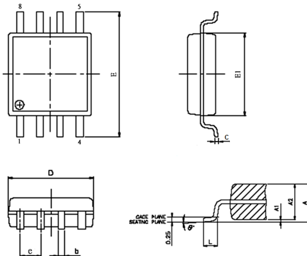
Figure 41. 8-pin SOP 200 mil (official name = 208 mil)
