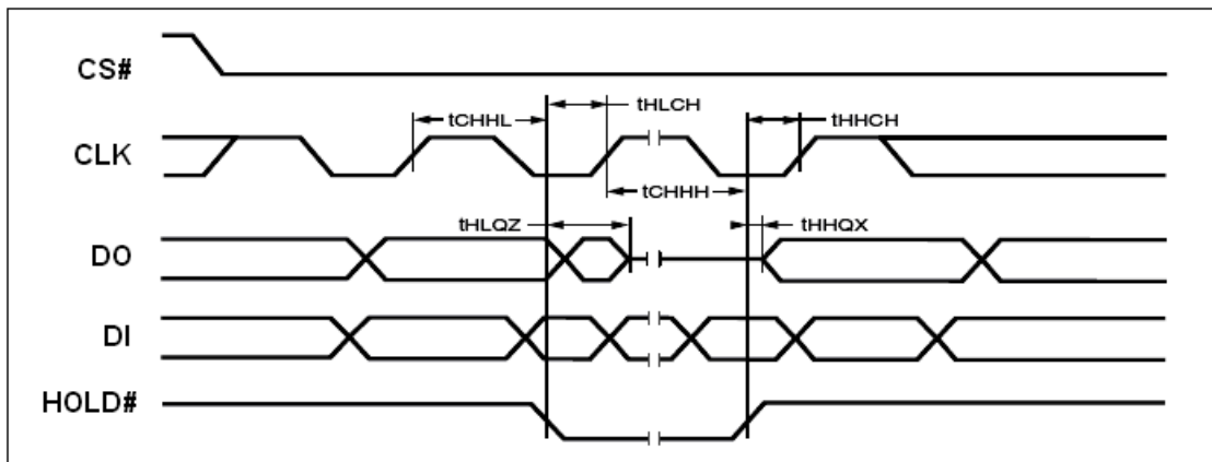
Figure 111. Hold Timing
