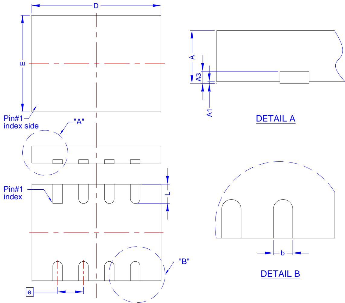
Figure 52. 8-contact USON (4x3x0.55 mm) without expose metal pad
