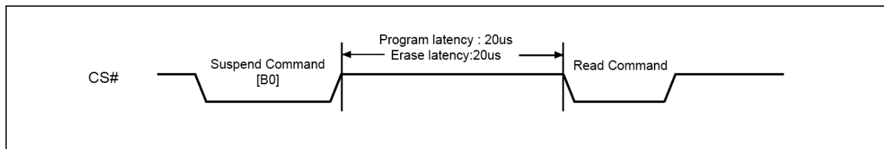
Figure 28.1 Suspend to Read Latency
