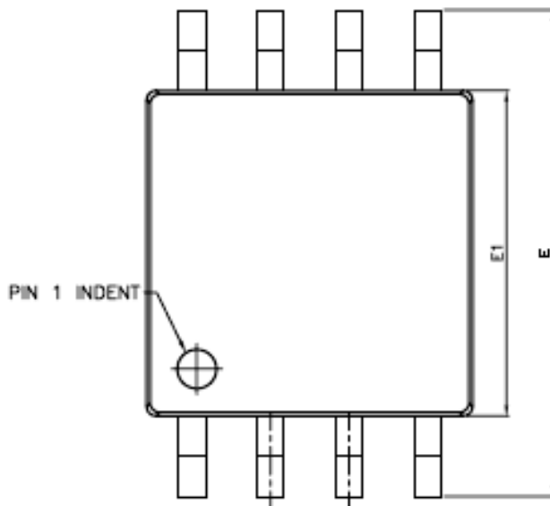
Figure 49. 8-pin VSOP 200 mil (Official name = 208 mil)
