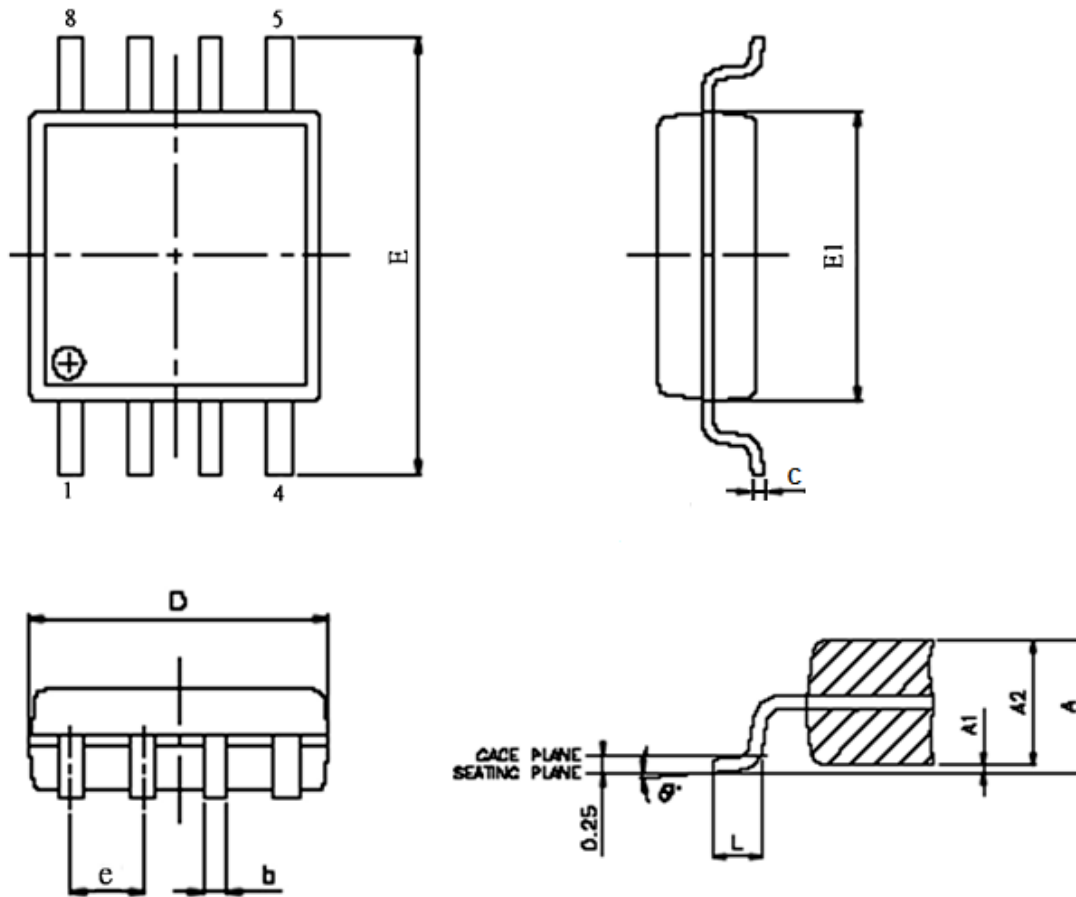
Figure 48. 8-pin SOP 200 mil (official name = 208 mil)
