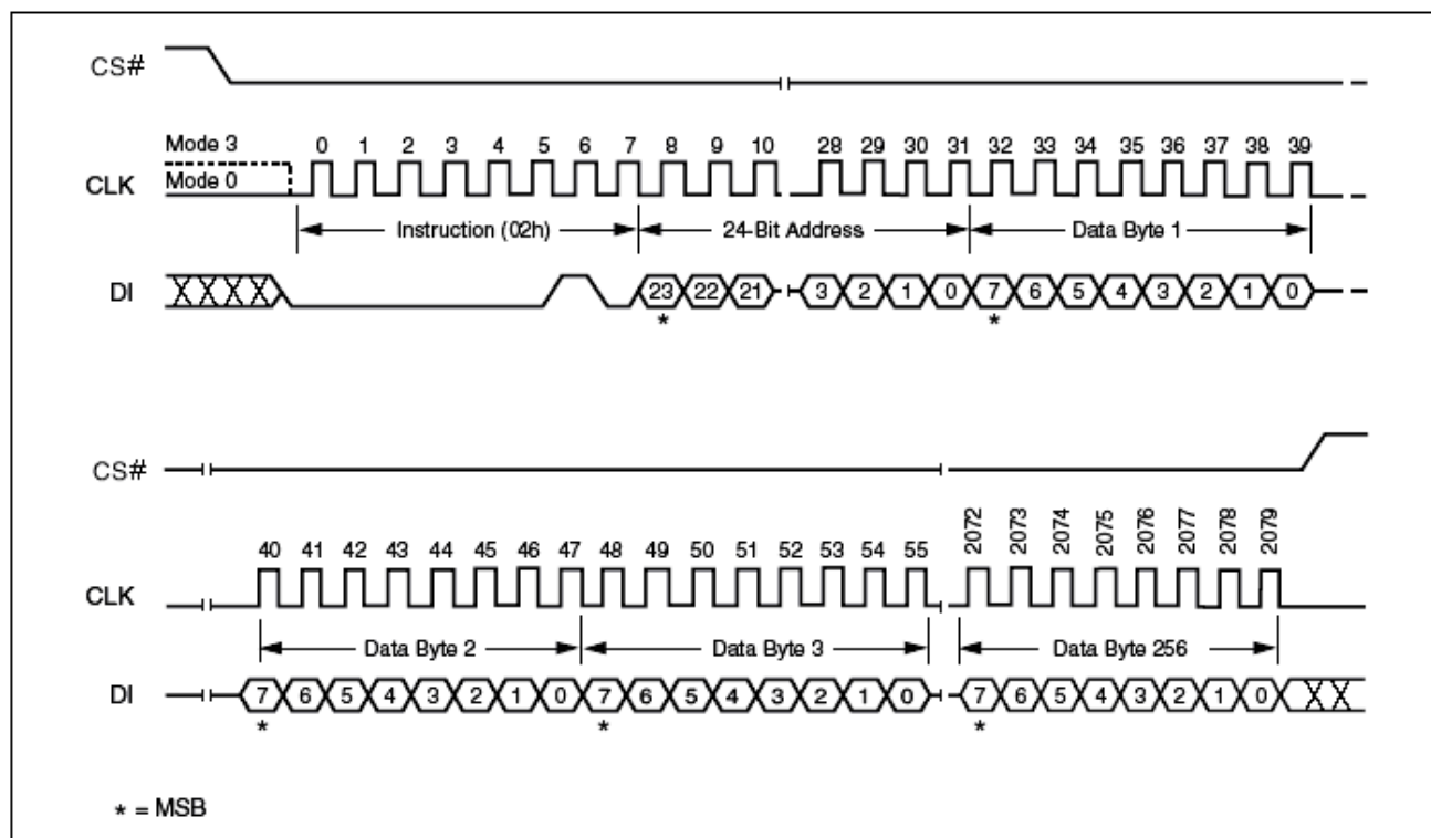
Figure 25. Page Program Instruction Sequence Diagram
