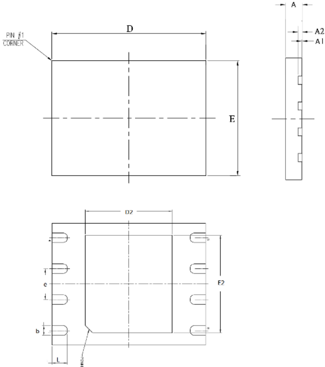
Figure 50. 8-contact VDFN (5x6mm)
