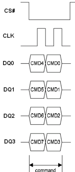
Figure 29.1 Write Suspend/Resume Instruction Sequence in QPI Mode
