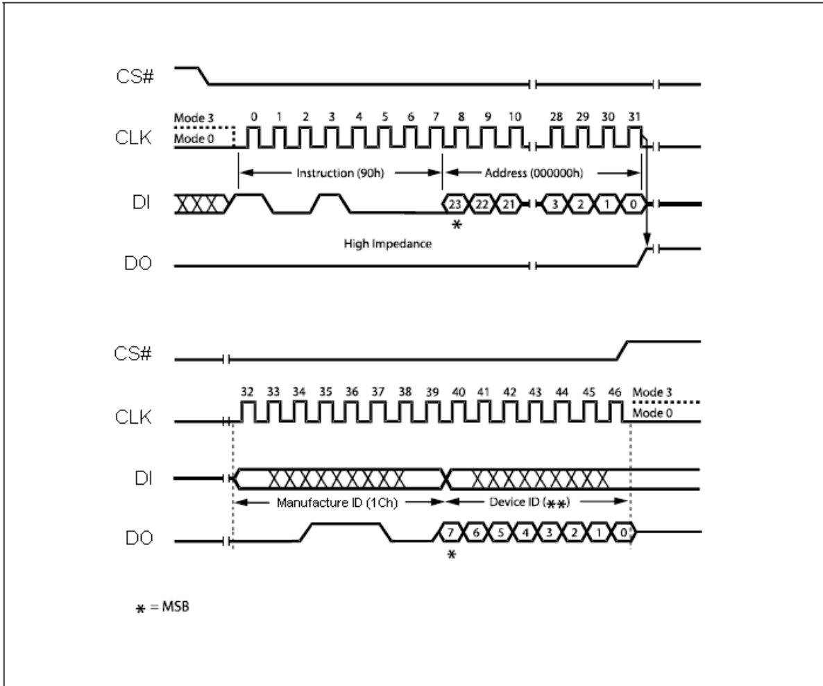
Figure 38. Read Manufacturer / Device ID Diagram
