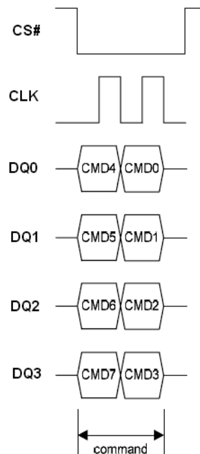
Chip Erase Sequence under EQPI Mode
