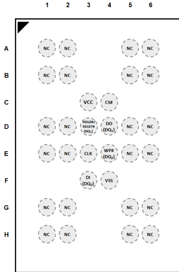
WLCSP (Package Code: SP)
