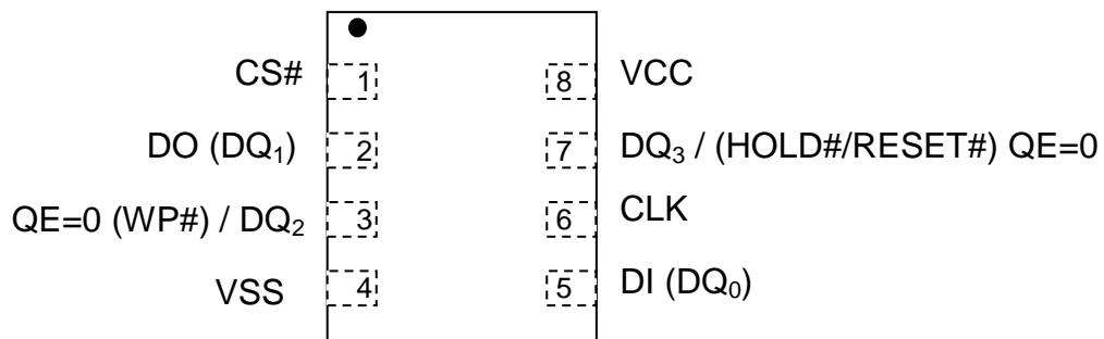
8 – LEAD VDFN / WSON
