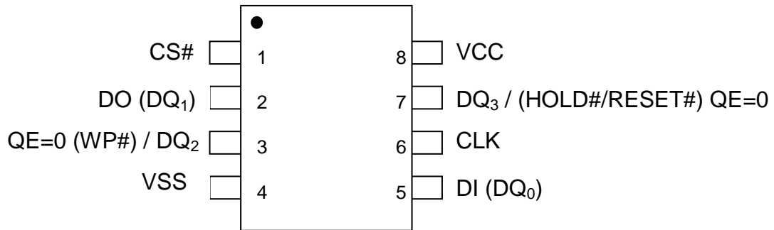
8 - LEAD SOP
