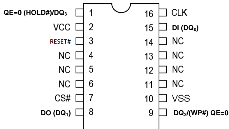
16 – LEAD SOP
