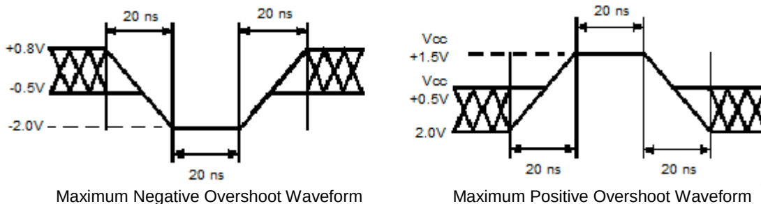
Figure 115. Overshoot Waveform
