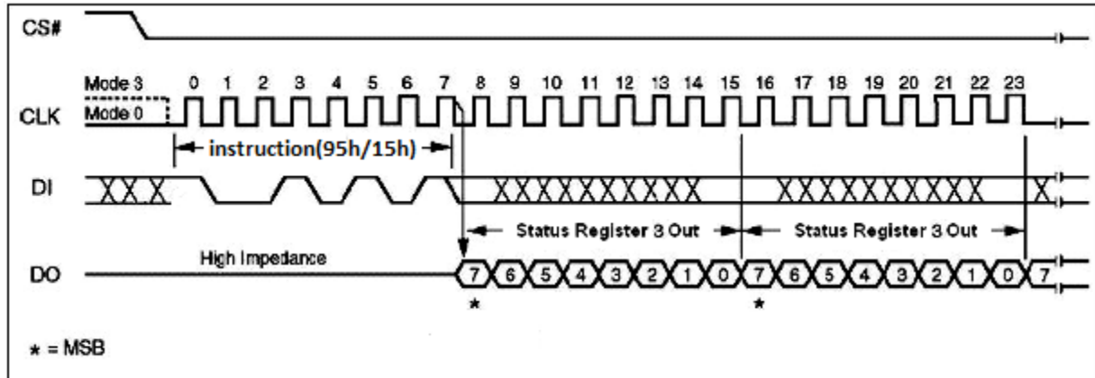
Figure 18. Read Status Register 3 Instruction Sequence Diagram
