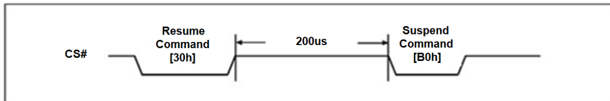
Figure 70. Resume to Suspend Latency
