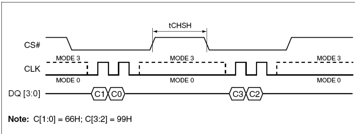
Figure 7. Reset-Enable and Reset Sequence Diagram under QPI Mode
