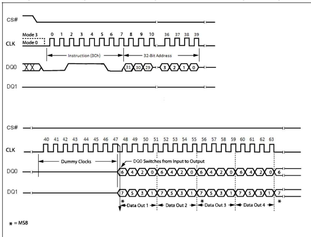
Figure 35. Dual Output Fast Read with 4byte address Instruction Sequence Diagram
