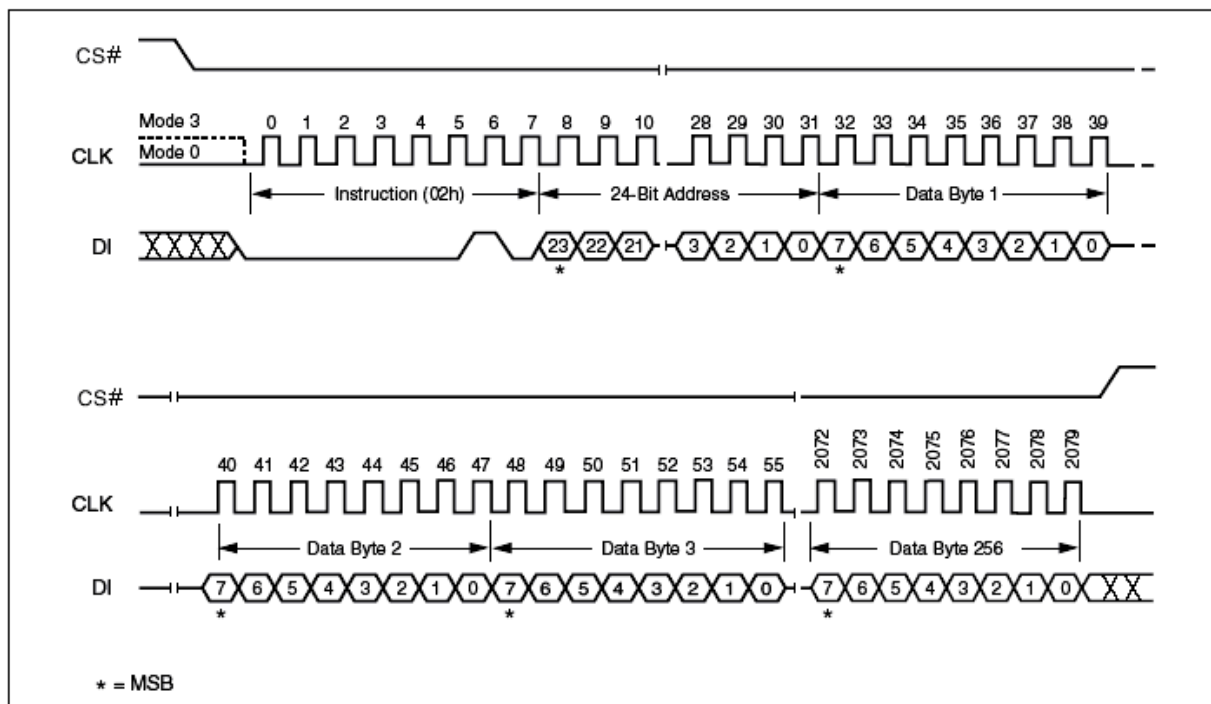
Figure 59. Page Program Instruction Sequence Diagram
