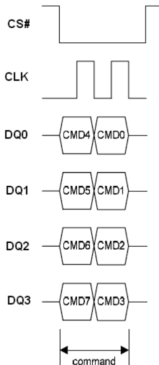
Figure 85. Enter 4byte address mode Sequence under EQPI Mode
