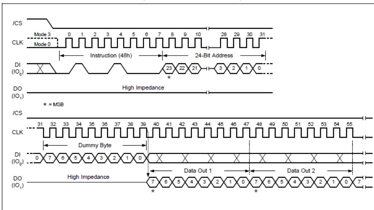
Figure 103. Read OTP array
