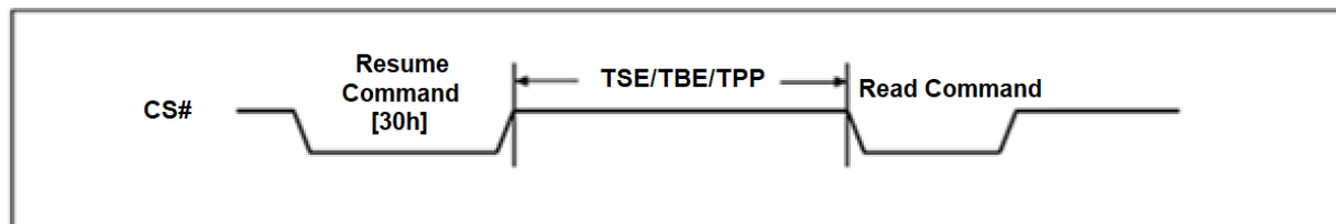
Figure 69. Resume to Read Latency
