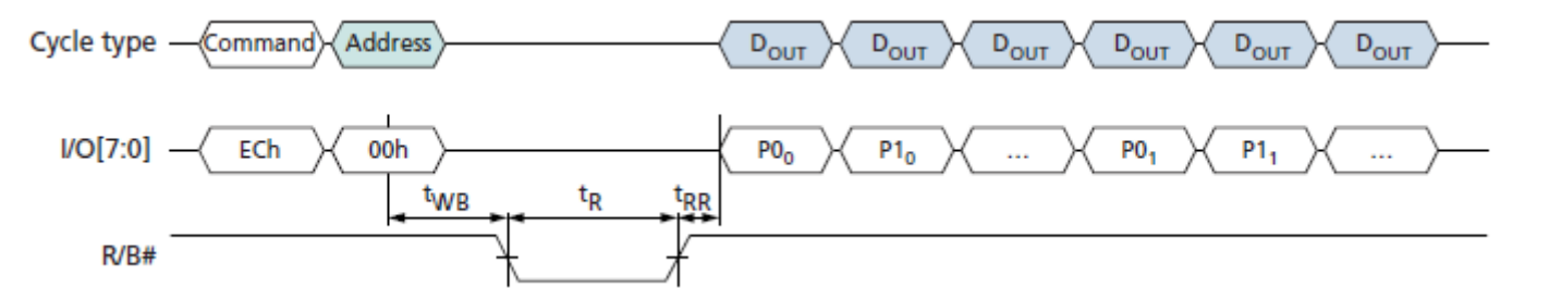
READ PARAMETER (ECh) Operation
