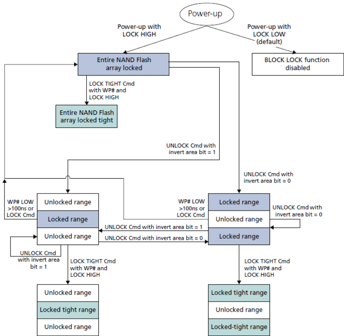
BLOCK LOCK Flowchart
