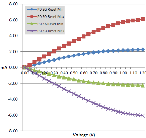
I-V Curve After ZQ Reset
