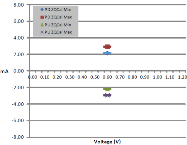
I-V Curve After Calibration
